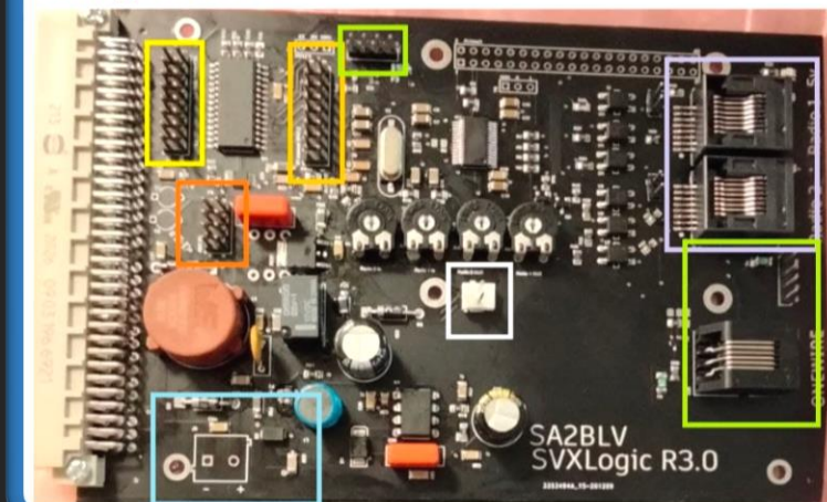
SvxLogic 3.0 / 3.1
